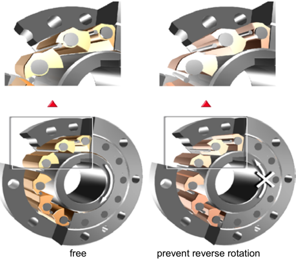
Conveyer Drives
