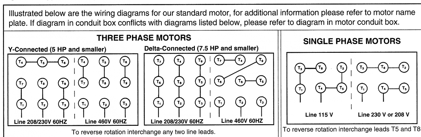
Fig. B-15 Typical Wiring Diagrams
