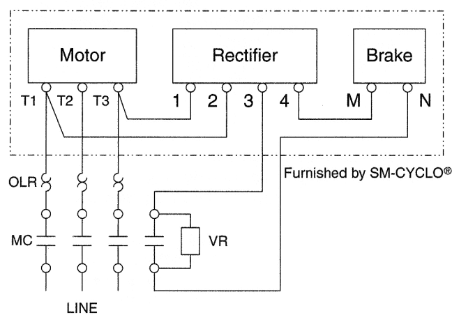
Fig. C-8d Fast Brake Action, Low Voltage
