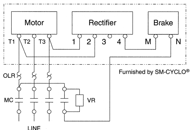
Fig. C-8b Fast Brake Action, High Voltage
