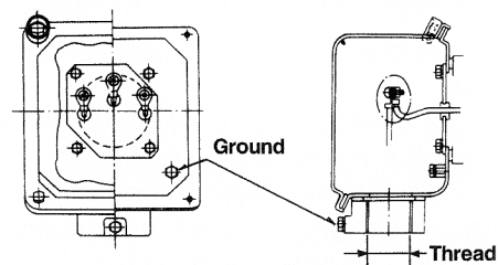
Fig. B-14 Weather-Proof Type
