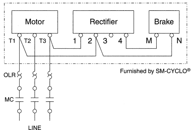
Fig. C-8a Normal Brake Action, High Voltage
