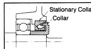
Fig. B-18 Slinger Type: Oil Lubed Units
