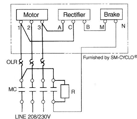
Fig. C-11c Low Voltage 200 ~ 230V
