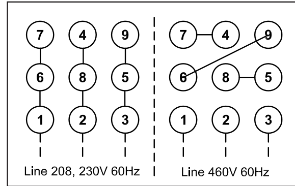
Figure 5.26 EP.NA - DELTA
