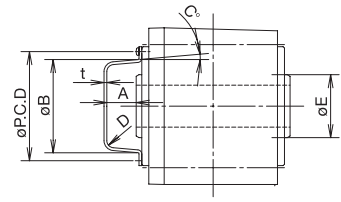
Figure 5.10 Frame Sizes 1200 ~1600
