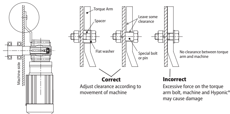
Figure 5.13 Hyponic® Torque Arm Clearance
