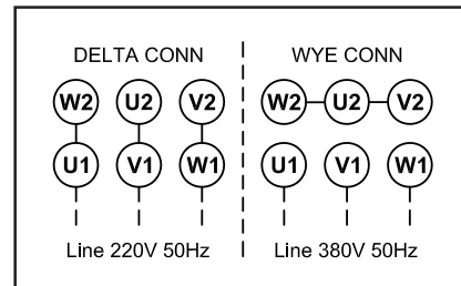
Figure 4.28 DELTA-WYE Diagram
