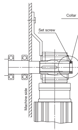
Figure 5.7 Secured by Set Screw and Collar
