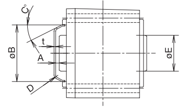
Figure 5.9 Frame Size 1100
